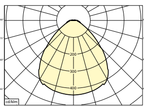
MS05223030 52W 5400lm 3000k 60° ηLB 59%
